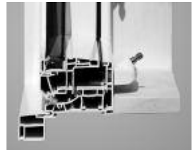
With the brickmould exterior option and an interior jamb extension the overall depth can be increased to 12-1/2".
